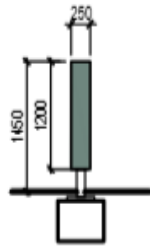
Side Elevation - North Street
