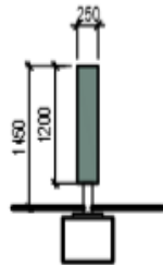
Side Elevation - Burgess Street
